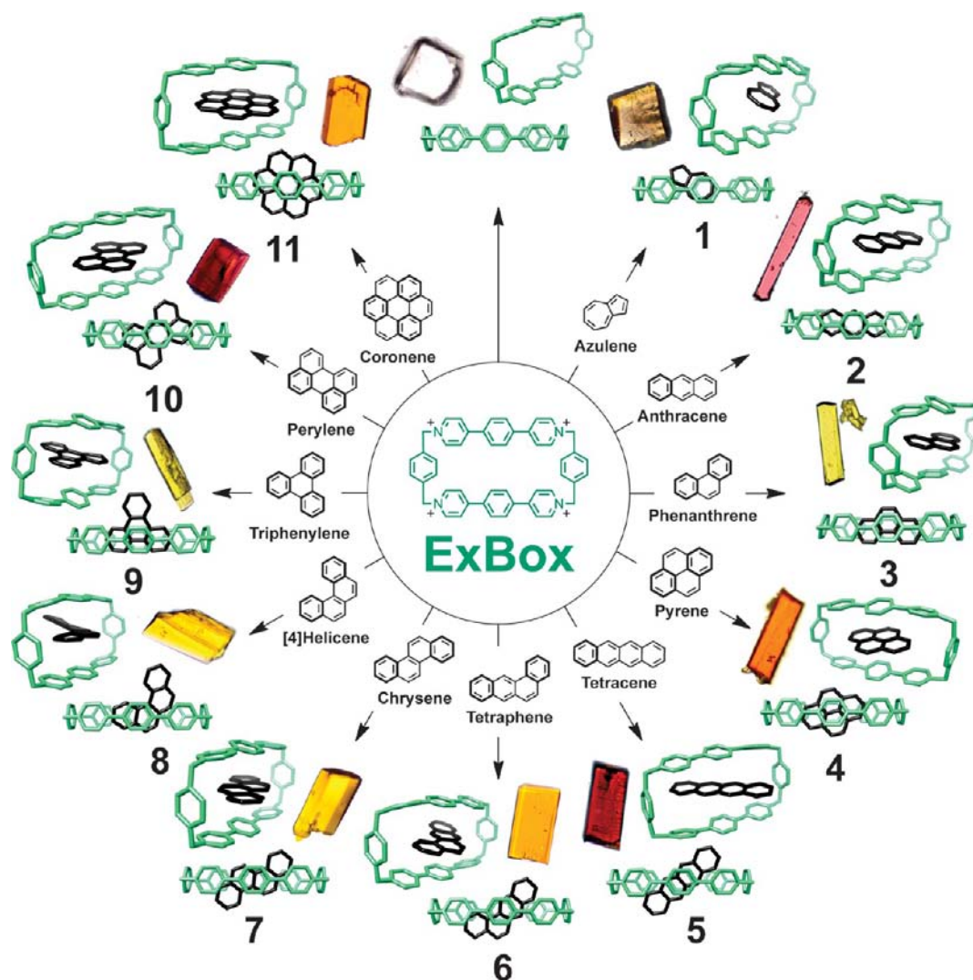
Figure 1. Single-crystal XRD data were obtained for all 11 of the inclusion complexes of \text{ExBox} \cdot \text{Cguest} \cdot 4\text{PF}_6 (1–11), along with that of \text{ExBox} \cdot 4\text{PF}_6 alone (top). The counterions and solvent molecules are removed for the sake of clarity. In each case, the crystals that were used to obtain the XRD data were photographed under an optical microscope. It is important to note the lack of color in the crystal of \text{ExBox} \cdot 4\text{PF}_6 by itself and the presence of different colors for each inclusion complex. The colors arise from charge-transfer interactions between the host and guests, with the exception of 1 because no charge-transfer band was observed in the optical absorption spectrum. The structural formulas depicted with bolded \pi -bonds highlight the Clar's sextet in each \pi -electron-rich guest.
