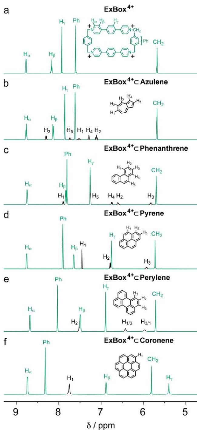
Figure 3. Aromatic-region insets of the ^1\text{H} NMR spectra of \text{ExBoxC}4\text{PF}_6 (a) and its 1:1 complexes with azulene (b), phenanthrene (c), pyrene (d), perylene (e), and coronene (f) recorded in \text{CD}_3\text{CN} at 298 K on a 500 MHz instrument. Upfield shifts of the \beta and \gamma protons of \text{ExBox}^{4+} as well as downfield shifts of the phenylene protons of \text{ExBox}^{4+} are evident. Both downfield and upfield shifts increase as the size of the PAH core becomes larger and larger, indicating the binding of a PAH molecule inside \text{ExBox}^{4+} in solution.
